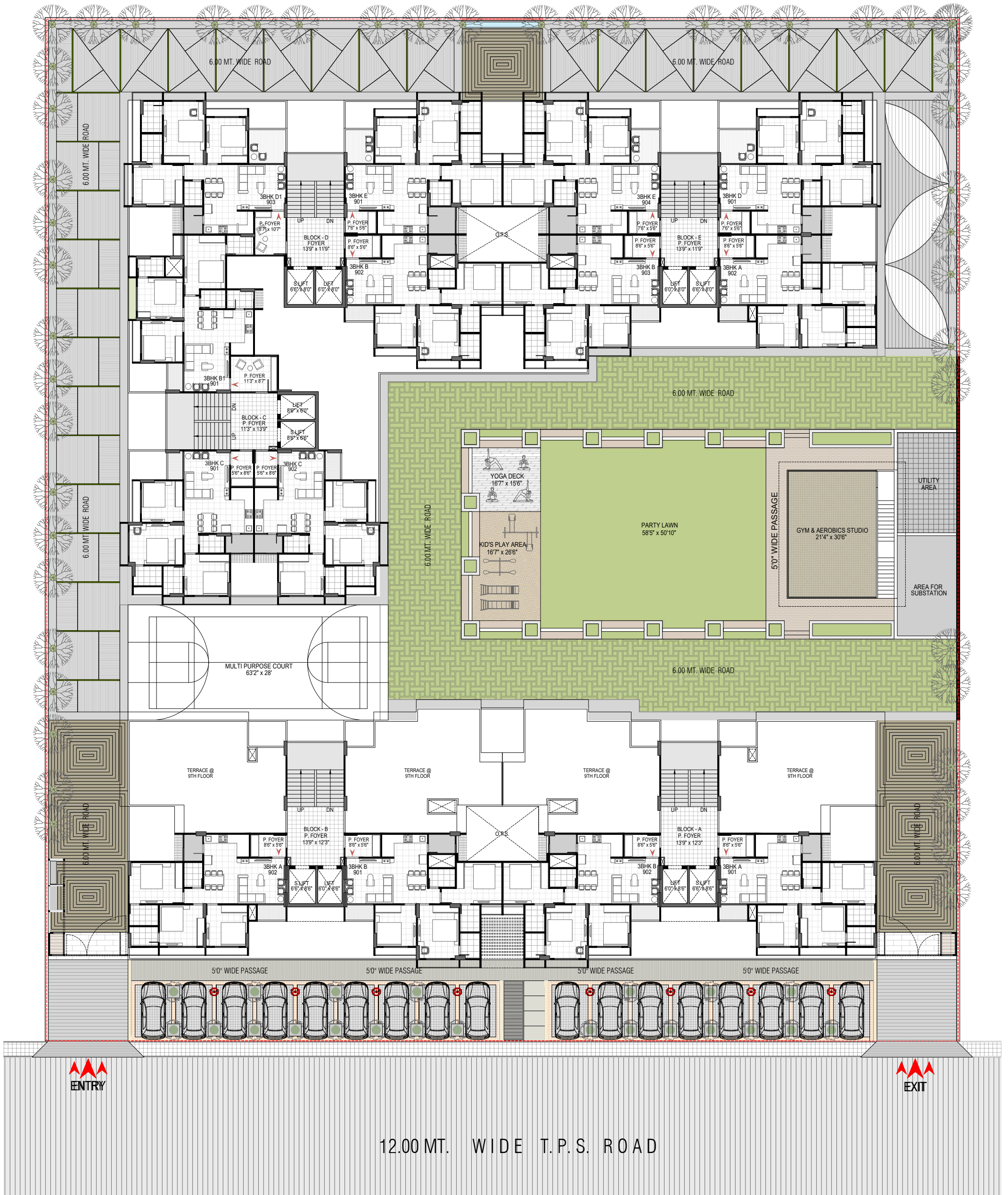
9th floor plan
